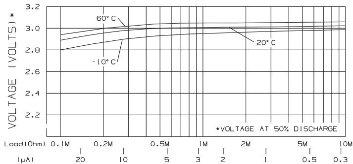
Operating Voltage v/s Load Resistance KCR2025
