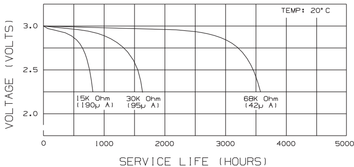
Typical Load Characteristics KCR2025
